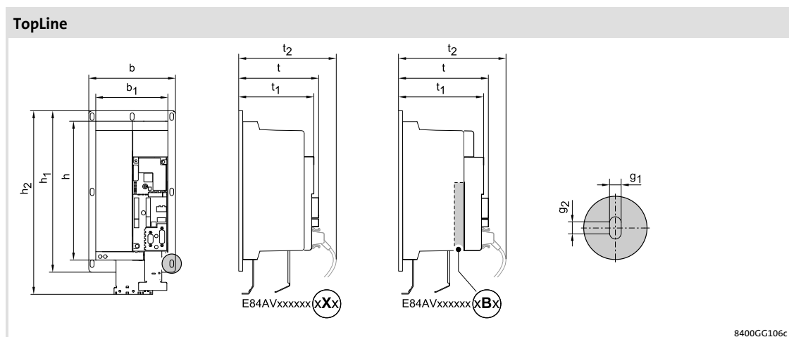
Fig. 5-35 Device dimensions
