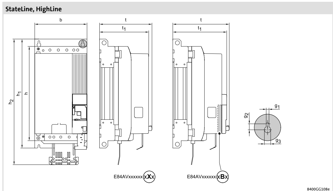
Fig. 5-41 Device dimensions
